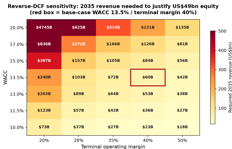
Figure 3: Reverse-DCF sensitivity: 2035 revenue (US$bn) required to justify the US$48.8bn equity value across WACC and terminal-margin assumptions. The red box marks the base case (13.5%/40%). Data: Table 9 in Appendix D.
